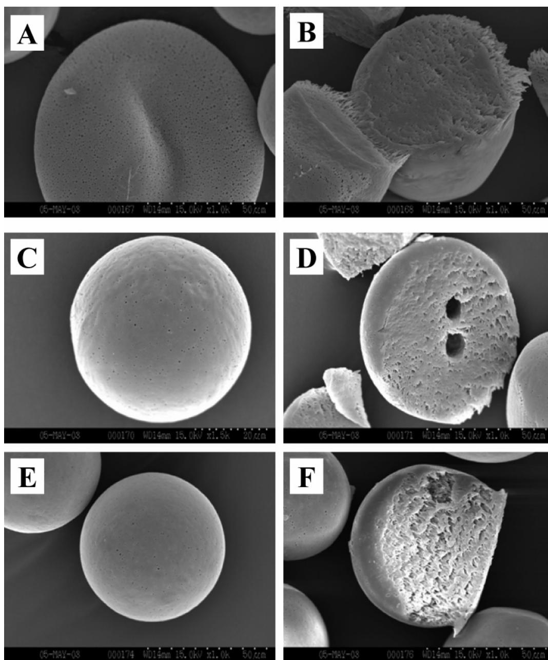
Figure 7. Scanning electron micrographs of the surface (left panel) and cross sections (right panel) of PLGA–Glu microsphere after incubation in PBST at 4 °C for 2 days (A and B) or at 37 °C for 2 h (C and D) and 2 days (E and F).
