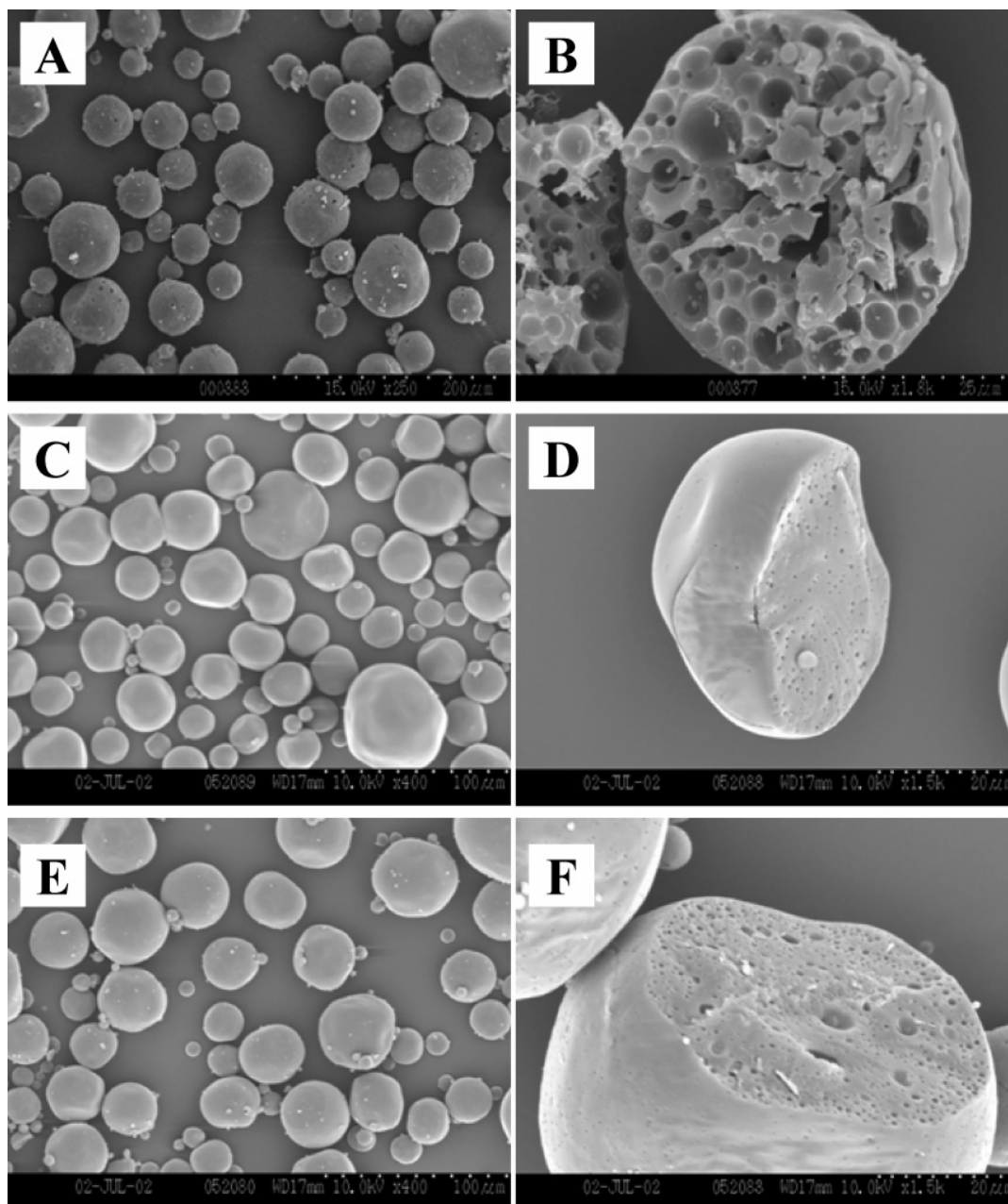
Figure 2. Scanning electron micrographs of the surface (left panel) and cross-section (right panel) of PLGA microspheres of formulation A (A and B), B (C and D), and C (E and F). The detailed formulation variables are listed in Table 1.
